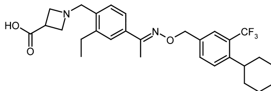
Figure 1 Chemical structure of BAE312.
